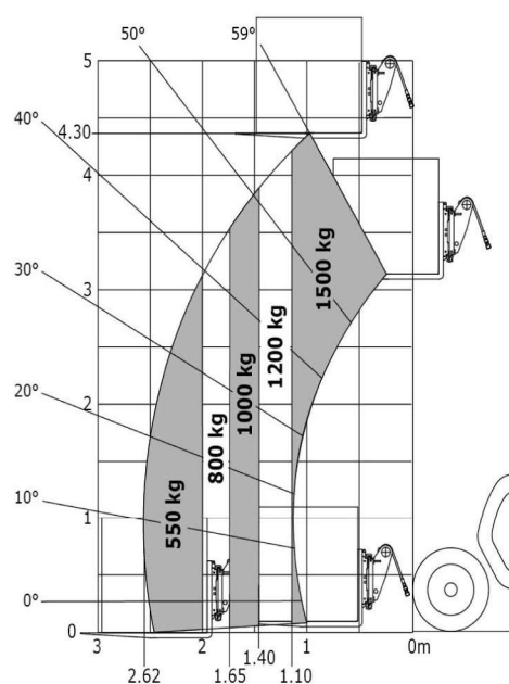
ULM 415 H
